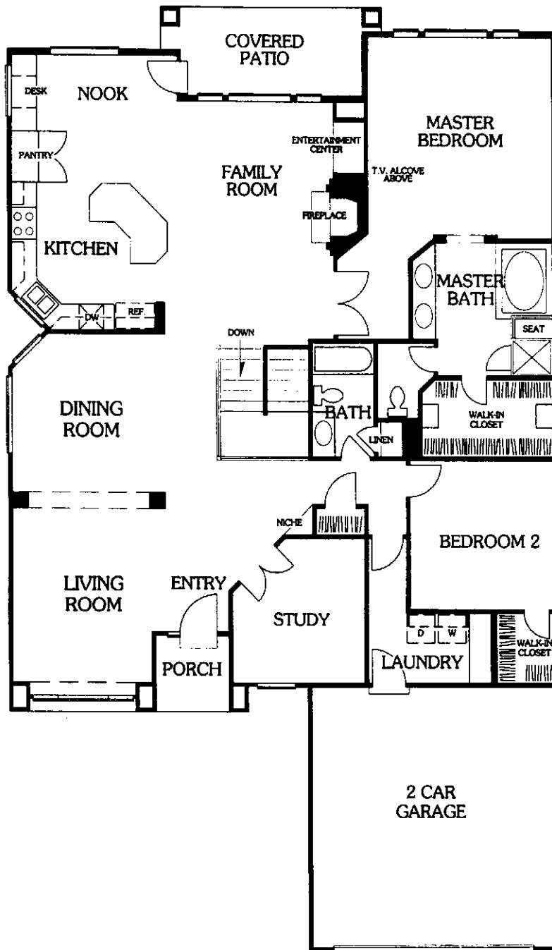
FIRST FLOOR
